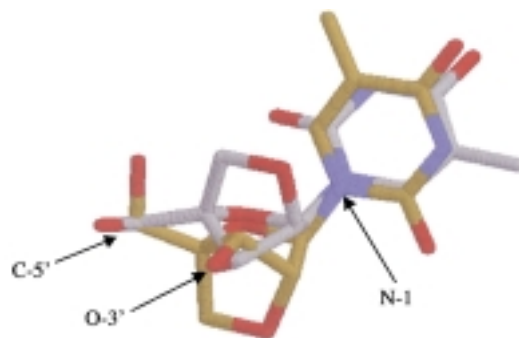
Figure 4. Energy-minimized structures of the LNA thymine nucleoside (yellow) and the \alpha -L-LNA thymine nucleoside (gray) (HyperChem program, Polak-Ribiere algorithm).
